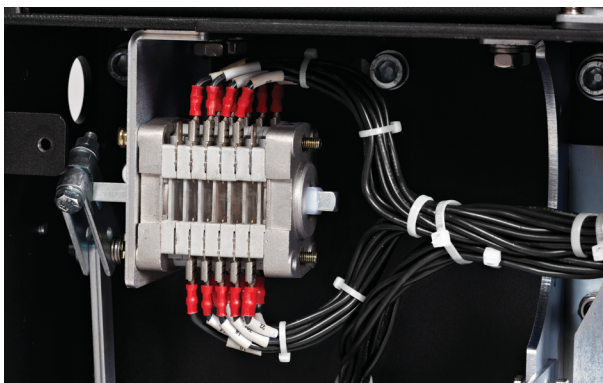
Auxiliary Switch
