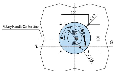
Front Contact Type
